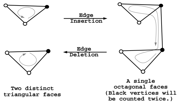
Figure 6. Inserting an edge between two different faces merges the two faces and deleting an edge with both sides in the same face splits the face into two.
