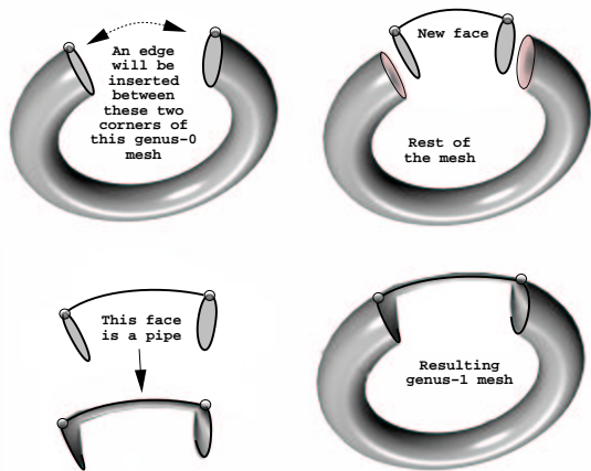
Figure 7. A multiple-step representative illustration of creating handle by inserting an edge. (Note that cutting off a handle can be considered the reverse order of this process).
