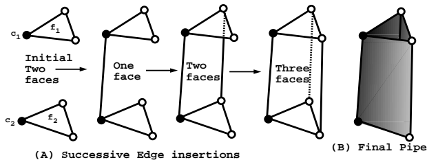
Figure 8. Creation of a high quality handle/hole by inserting a set of edges.
