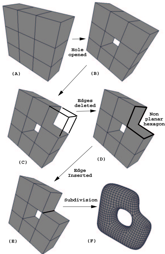
Figure 10. Modeling a simple 2-manifold that looks like a non-manifold.
