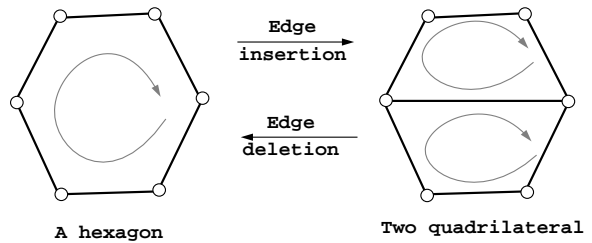
Figure 5. Inserting an edge between two corners of the same face divides it into two faces and deleting an edge between two faces merges the two faces into one.
